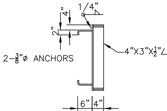
GRATING TYPE B
