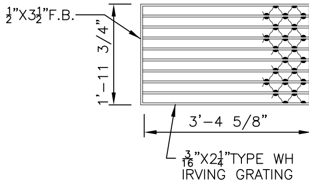
GRATING TYPE B
