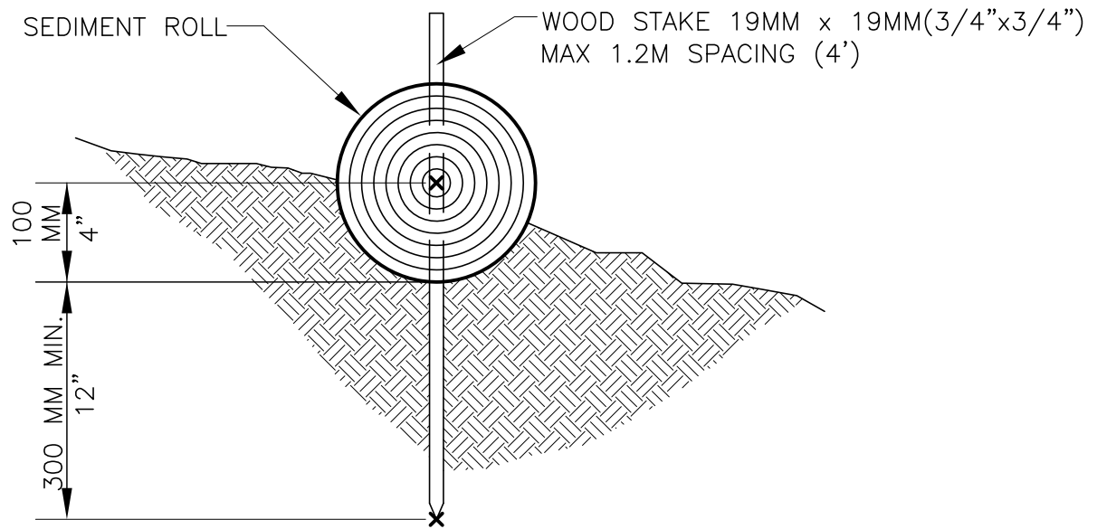
ENTRENCHMENT DETAIL IN SLOPE AREA N.T.S.
